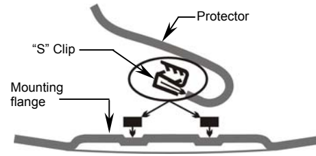
Illustration #3: Clip Configuration
