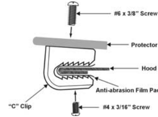
Illustration #3: Clip Configuration
