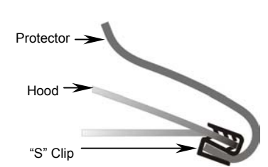
Illustration #2: "S" Clip Installation on Hood
