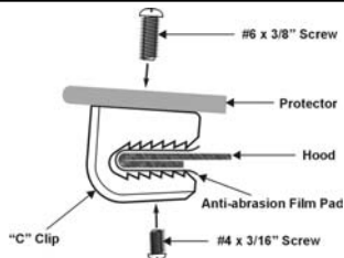
Illustration #3: Clip Configuration
